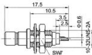
mounting hole
