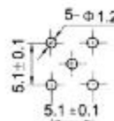
mounting hole
