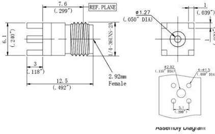
Assembly Diagram
