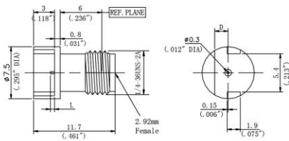
Assembly Diagram
